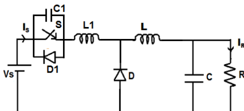
Figure 1. Graphical schematic of the ZVS Buck converter.
