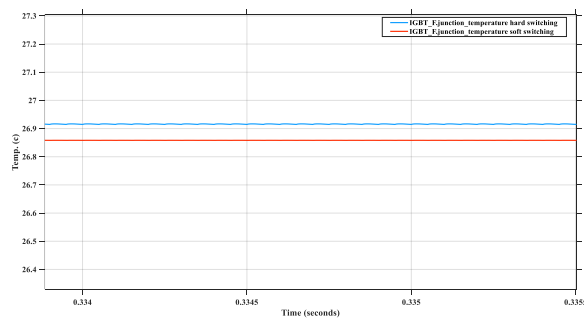
Figure 5. Soft and Hard switching junction temperature.
