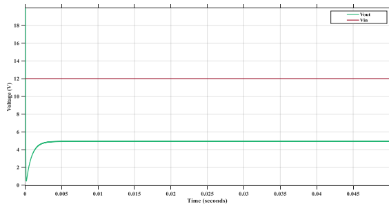
Figure 4. Input and output voltages.
