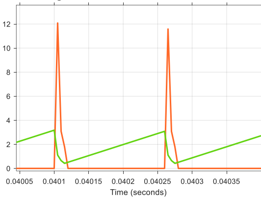
Figure 3. Soft switching V_{ce} and I_{ce} .
