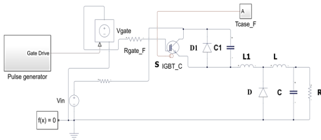
Figure 2. Simscape Proposed Model
