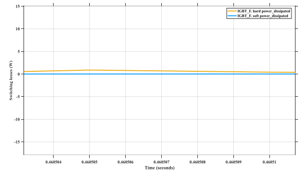
Figure 7. Soft and Hard switching losses.
