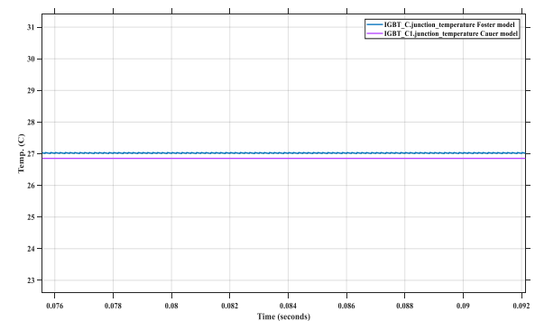
Figure 8. Cauer and Foster Models Junction Temp.
