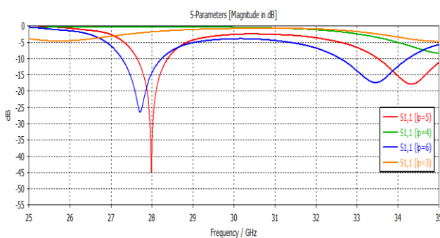
Fig. 4. Effect of changing patch length to the return loss
