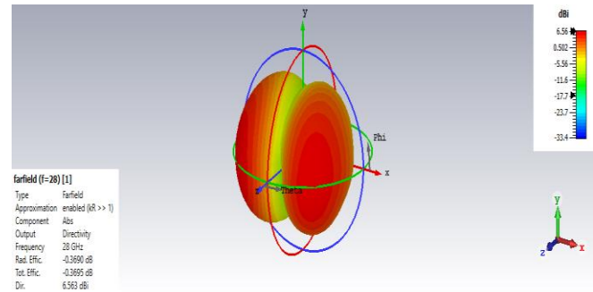
Fig.10. 3D plot of far-field directivity at 28GHz
