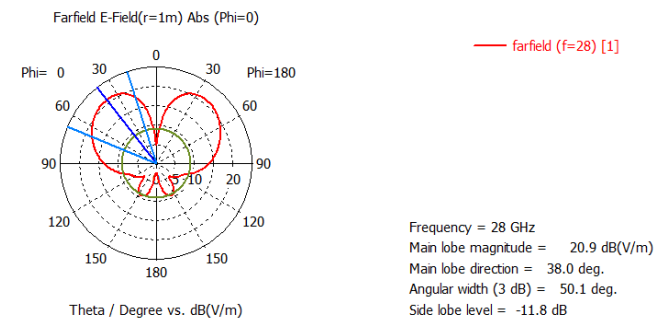
Fig.11. Polar plot of Far-field E –field pattern at 28 GHz
