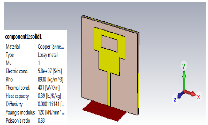
Fig. 2. 3D View of the Suggested Microstrip Patch Antenna
