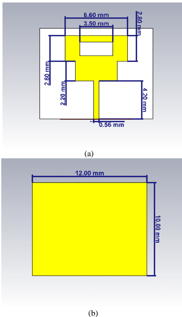
Fig. 1. The Suggested Antenna (a) Patch layer (b) Ground layer
