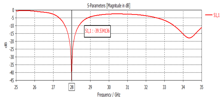
Fig. 6. Return Loss versus Frequency
