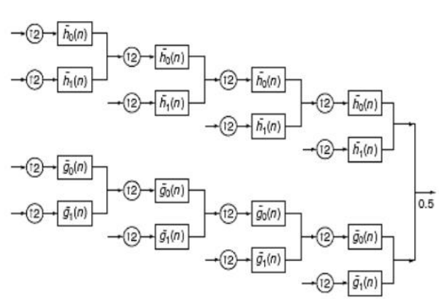
Fig. 3. Complex wavelet transform synthesizer filter.
