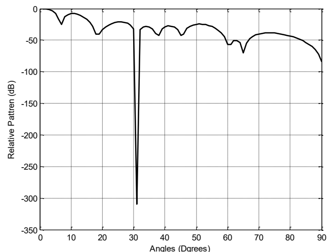
Fig. 10. Linear array pattern with one null and SLL=-18 dB.
