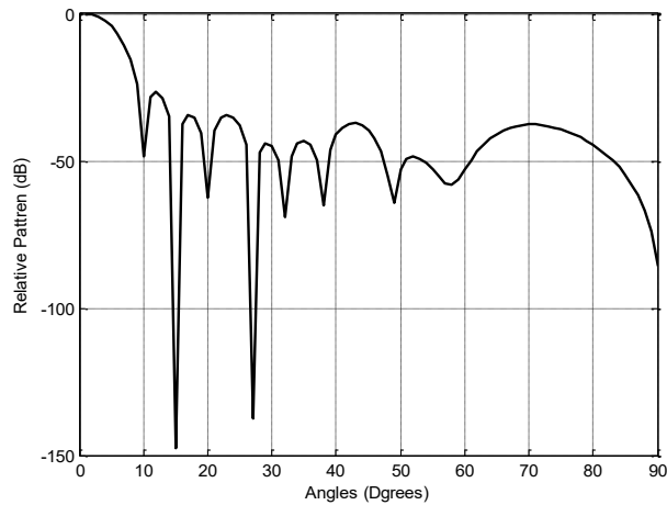
Fig. 12. Linear array pattern with 2 nulls and SLL=-30 dB.
