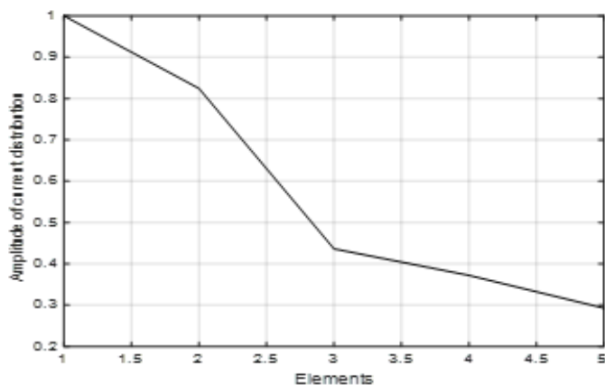
Fig. 11. Antenna array current distribution.
