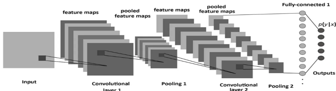
Fig. 1. An example of CNN [14]
